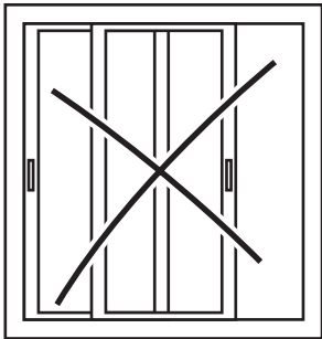
Sliding Window
